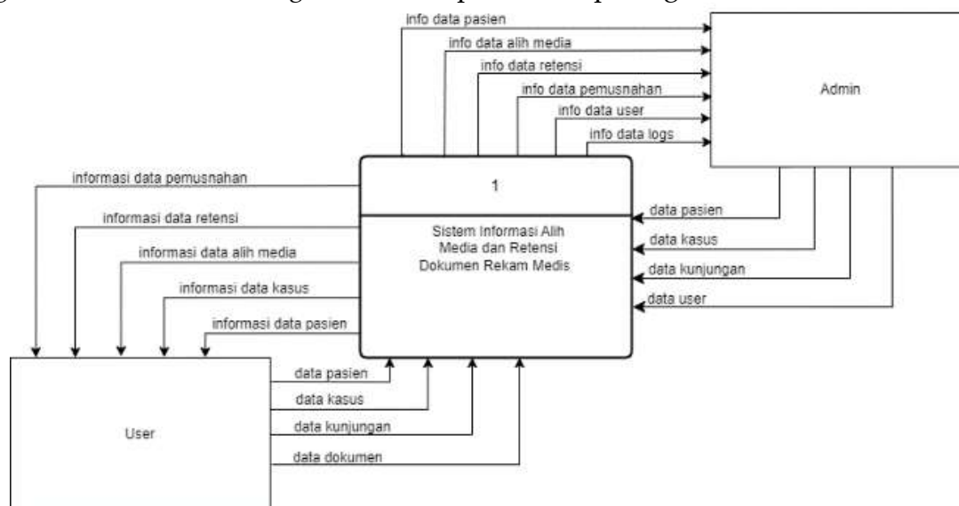
Gambar 2. Context Diagram
