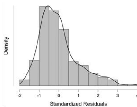
Gambar 1. Analisa Uji Normalitas Standardized Residuals Histogram
