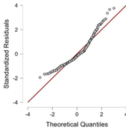
Gambar 2. Analisa Uji Linieritas Q-Q Plot Standardized Residuals
