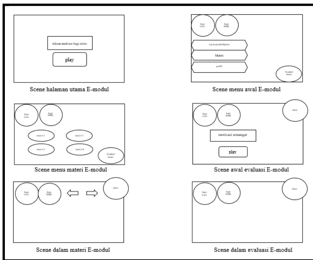
Gambar 3. Story Board
